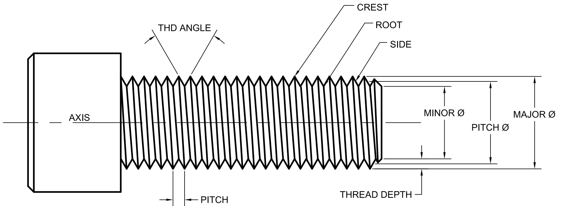
SCREW THREAD NOMENCLATURE EXTERNAL DETAILED THREAD
