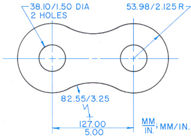
BICYCLE CHAIN LINK (FIG 3.06)
