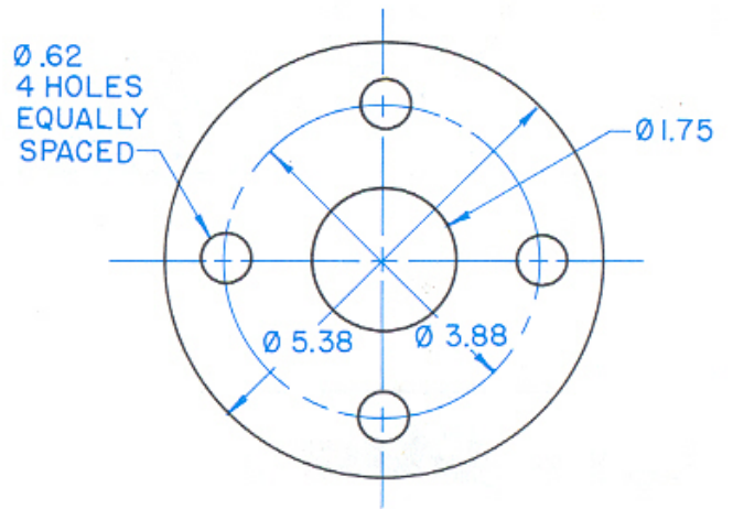
ROUND FLANGE (FIG 3.07)
