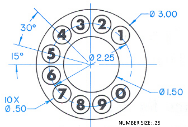
PHONE DIAL (FIG 3.09)
