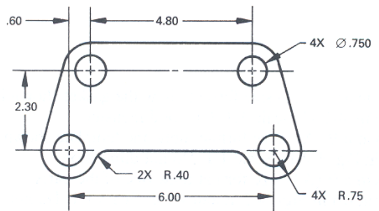
COVER PLATE (FIG 3.11)
