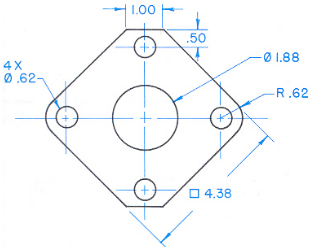
BRONZE PLATE (FIG 3.08)
