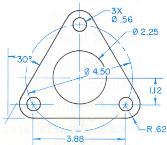
BASE PLATE (FIG 3.10)
