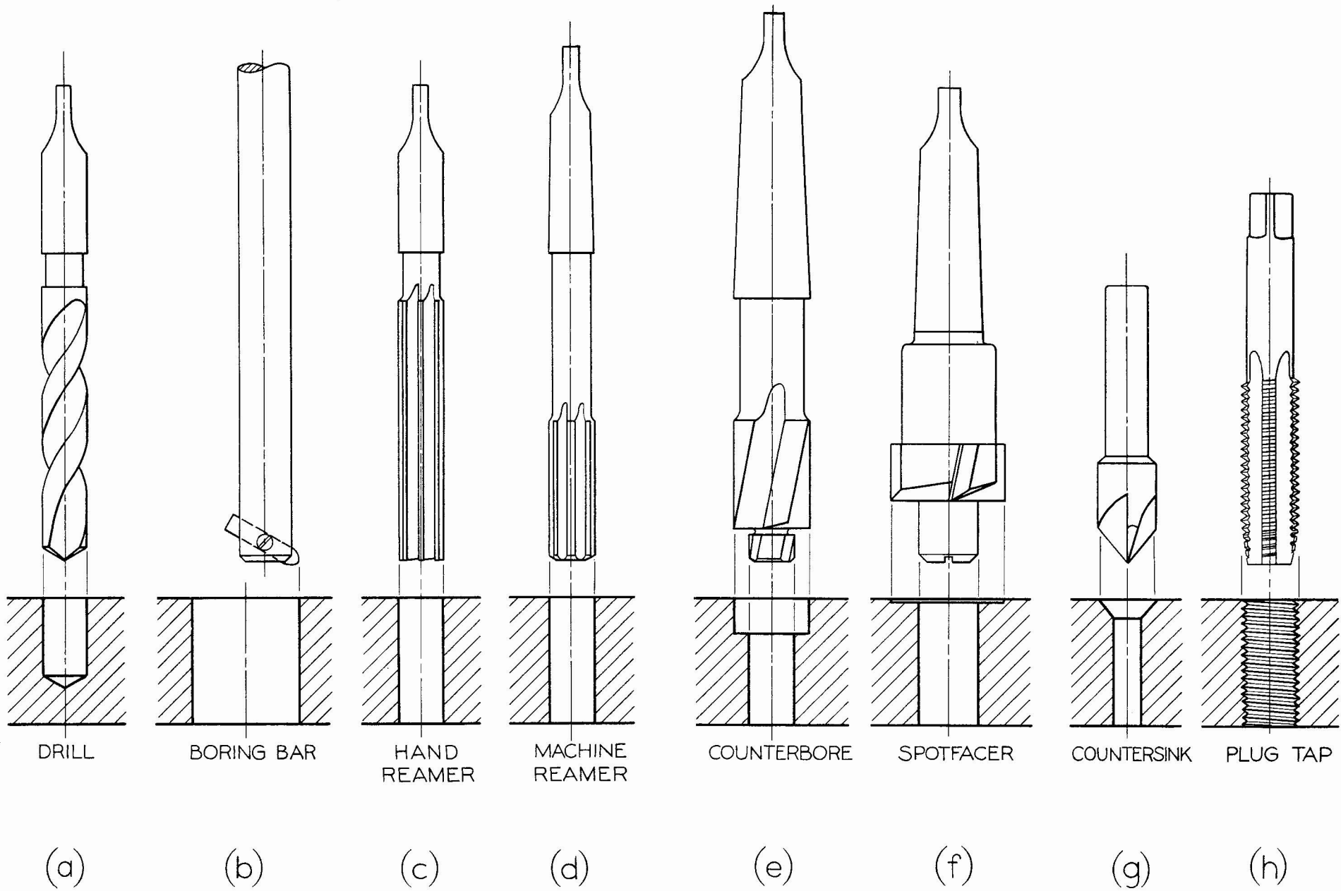
FIGURE 10.19 Types of Machined Holes.
